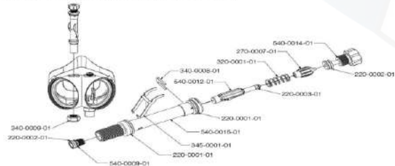
350M BIBS Mask Exhaust Regulator Assembly (540-0002-01)
